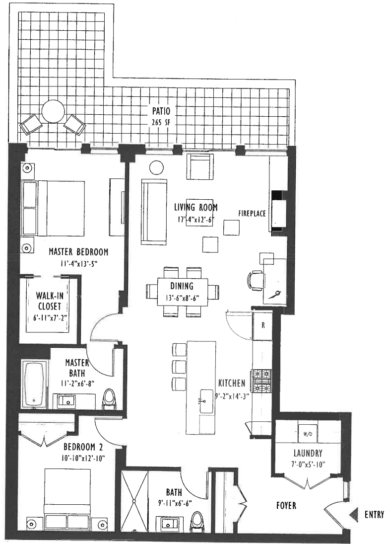
LEVEL 1 1395 SF
